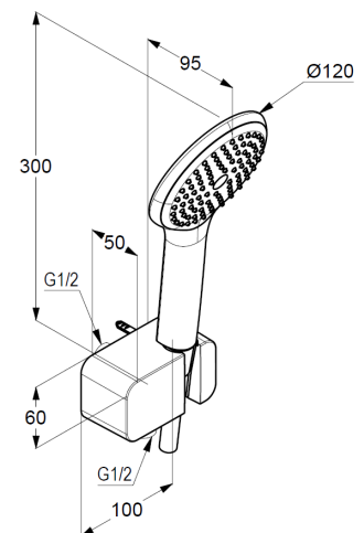
Dimensional drawing
