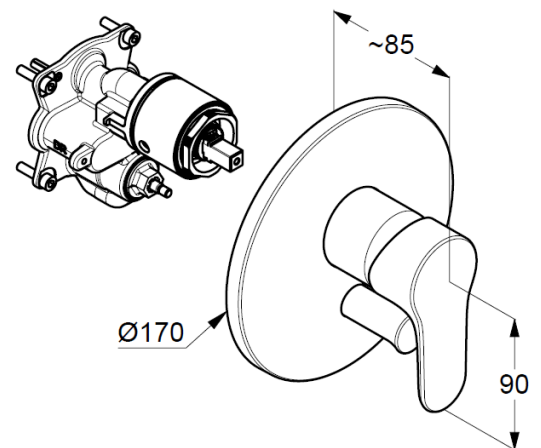
Dimensional drawing
