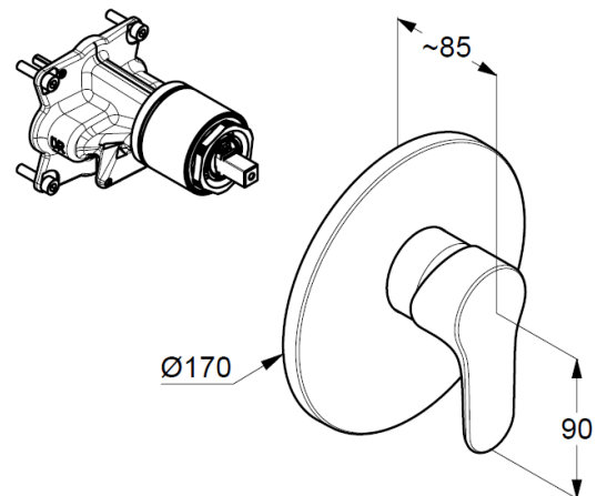
Dimensional drawing
