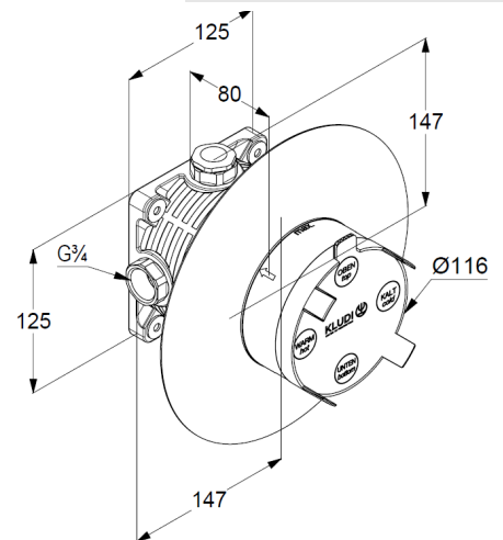
Dimensional drawing
