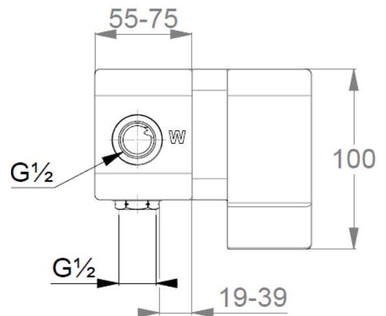
Dimensional drawing
