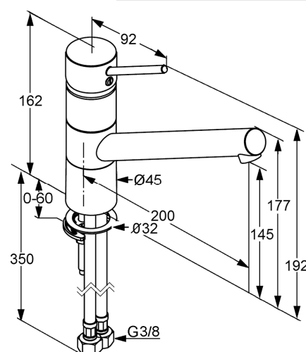
Dimensional drawing
