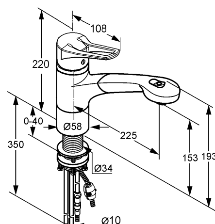
Dimensional drawing
