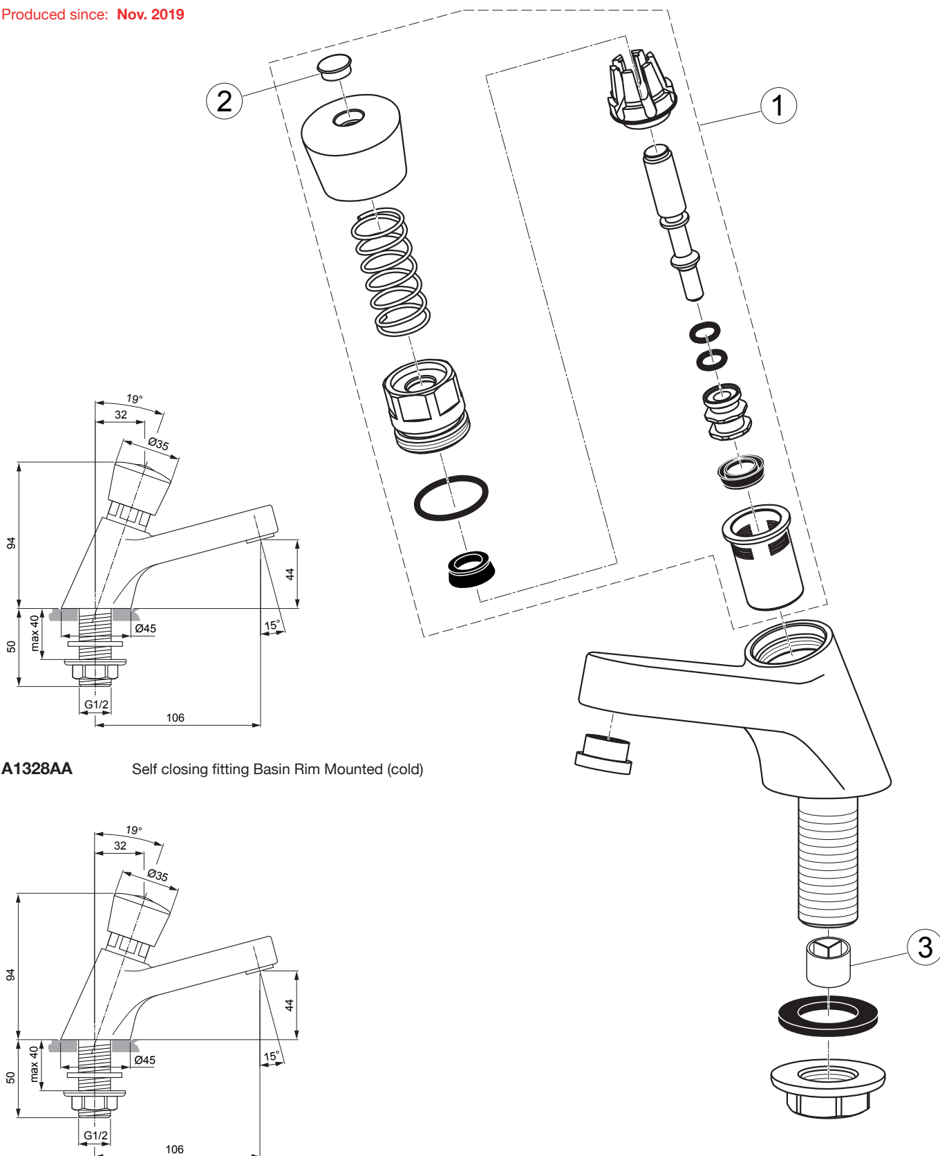
A1329AA Self closing fitting Basin Rim Mounted (hot)
