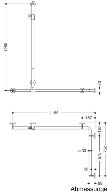
Abmessungen in mm
