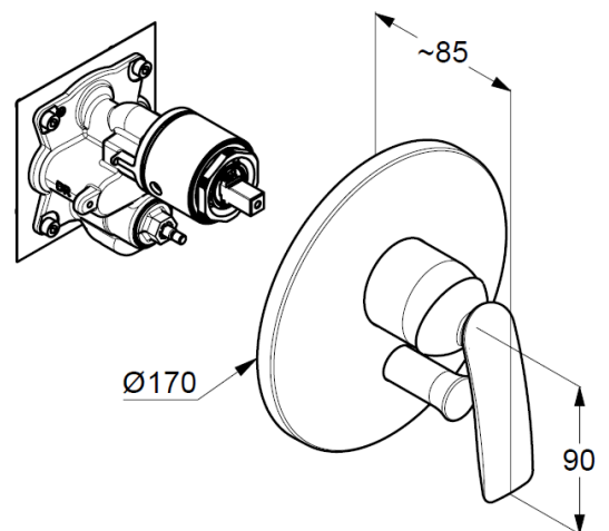
Dimensional drawing
