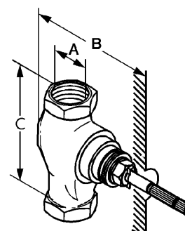
Dimensional drawing
